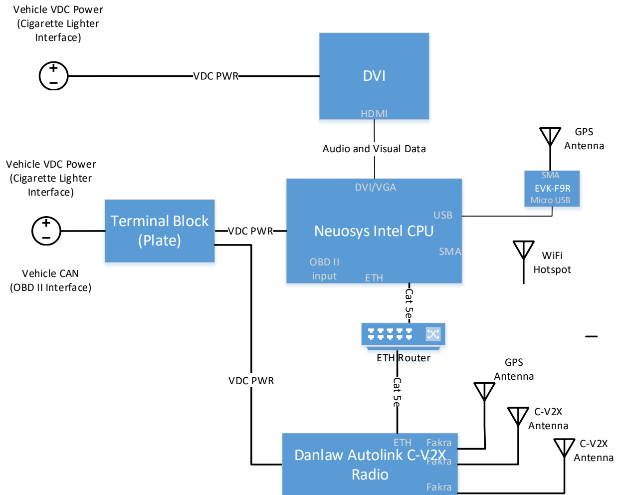
Figure 8. VBS Hardware Used for Field Test - (Source: Battelle)
